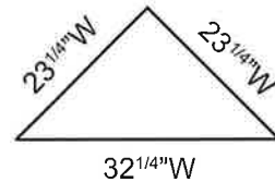
73272: Corner Cabinet 72"H x 32 1 / 4 "W x 16 1 / 4 "D 3 adjustable shelves
