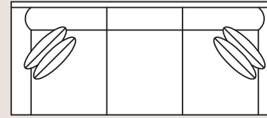
9100 Sofa Overall: H 38 W 94 D 40 Seating: H 19 W 80 D 24 Seat Height: 19 Arm Height: 26 Pillows: 4 P21
