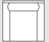
9101 Chair Overall: H 38 W 41 D 40 Seating: H 19 W 27 D 24 Seat Height: 19 Arm Height: 26
