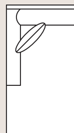
9182 LAF One Arm Chaise 9183 RAF One Arm Chaise Overall: H 38 W 36 D 64 Seating: H 19 W 29 D 48 Seat Height: 19 Arm Height: 26 Pillows: 1 P21
