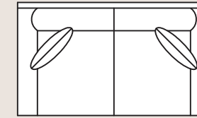
9120 Loveseat Overall: H 38 W 68 D 40 Seating: H 19 W 54 D 24 Seat Height: 19 Arm Height: 26 Pillows: 2 P21
